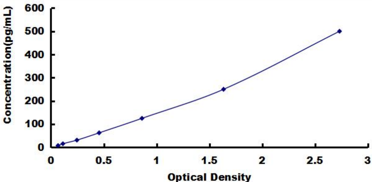
Typical Standard Curve for TNFa, Bovine ELISA.
