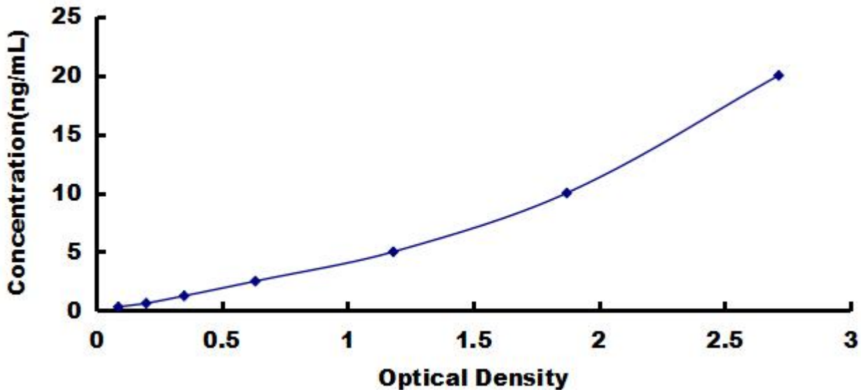
Typical Standard Curve for Vinculin, Mouse ELISA.
