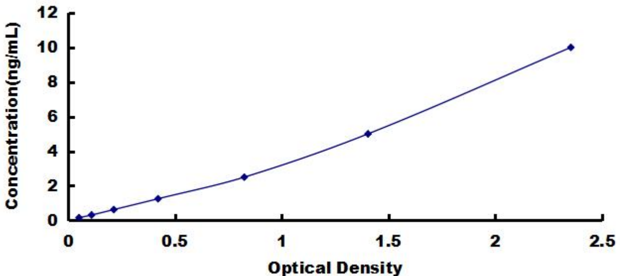
Typical Standard Curve for WNT3A, Human ELISA.
