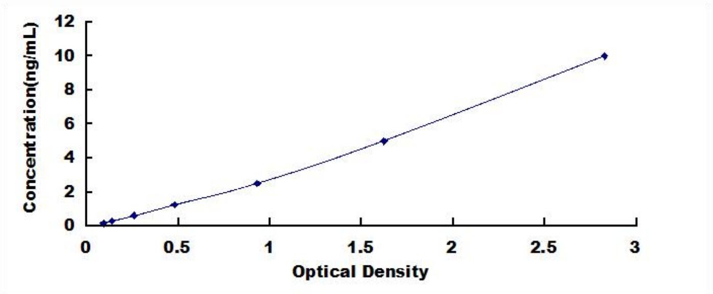
Typical Standard Curve for APOA4, Mouse ELISA.
