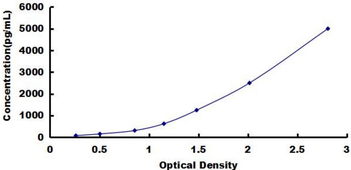
Typical Standard Curve for C5a, Mouse ELISA.
