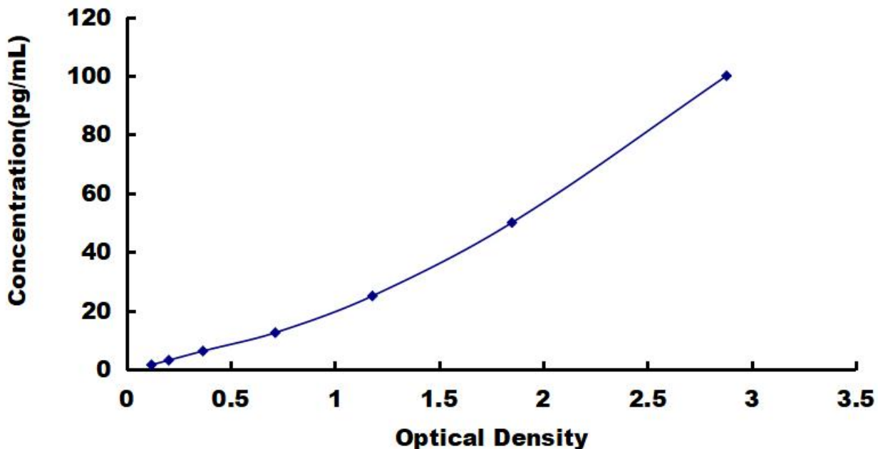
Typical Standard Curve for IL6, Rat ELISA.
