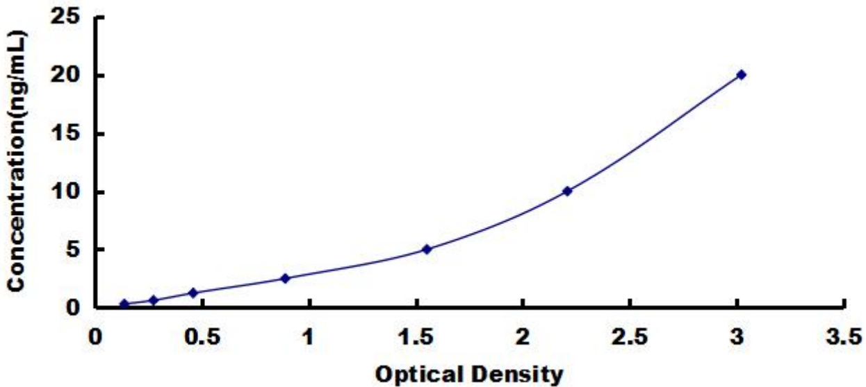
Typical Standard Curve for S100A4, Human ELISA.
