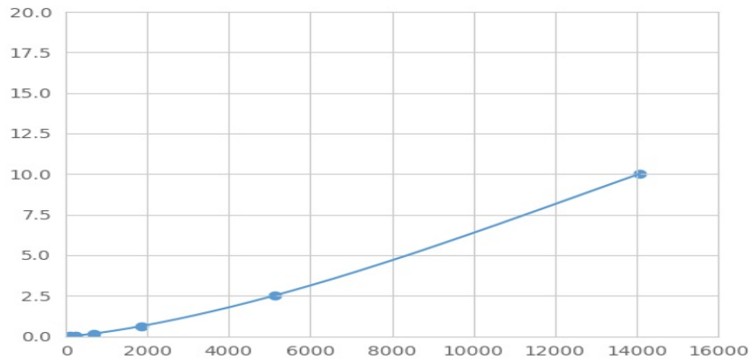
Typical Standard Curve for WNT3A Magnetic Luminex Assay.
