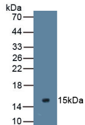
Figure. Western Blot; Sample: Recombinant MUC2, Human.
