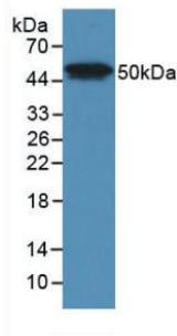
Figure. Western Blot; Sample: Recombinant LpPLA2, Human.
