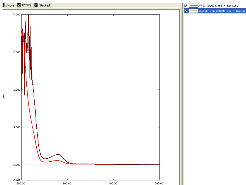
Figure 1. UV of the Original Peptide
