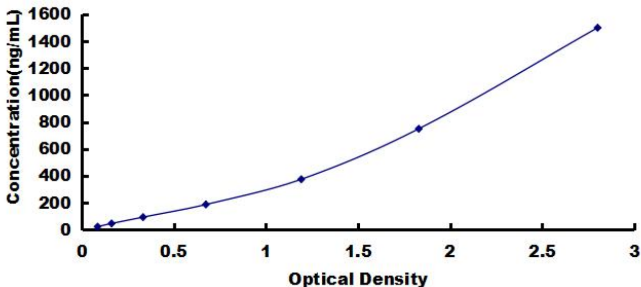
Typical Standard Curve for APOE, Human ELISA.
