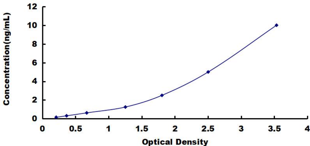
Typical Standard Curve for CST4, Human ELISA.
