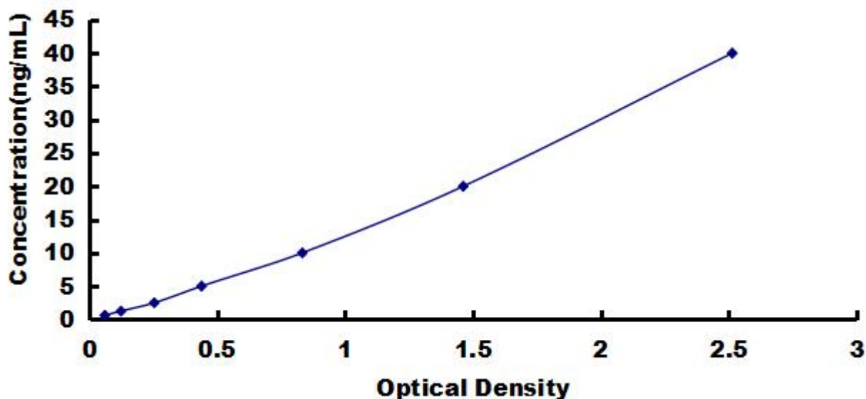
Typical Standard Curve for Cys-C, Mouse ELISA.
