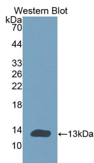
Figure. Western Blot; Sample: Recombinant CHRNa1, Human.
