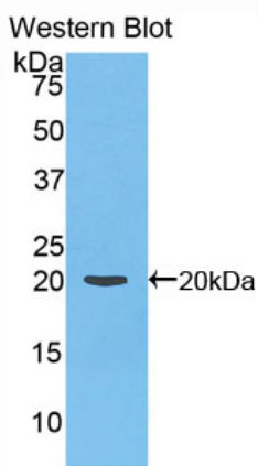
Used in Western Blot, Sample: Recombinant F2, Rat
