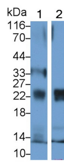
Western Blot; Sample: Lane1: Rat Liver lysate; Lane2: Porcine Liver lysate Primary Ab: 0.5µg/ml Rabbit Anti-Human GPX1 Antibody Second Ab: 0.2µg/mL HRP-Linked Caprine Anti-Rabbit IgG Polyclonal Antibody (Catalog: SAA544Rb19)
