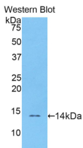
Figure. Western Blot; Sample: Recombinant RETN, Mouse.
