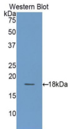
Figure. Western Blot; Sample: Recombinant TSPAN3, Human.
