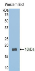
Figure. Western Blot; Sample: Recombinant TCF20, Mouse.
